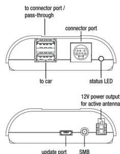
DAB+U installation diagram
